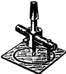
Circle cutter.
